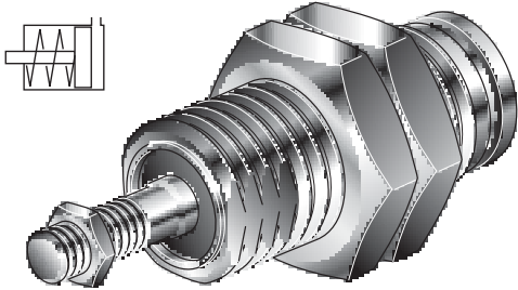
Minicylinder single acting front spring. Microcilindro semplice effetto molla anteriore
